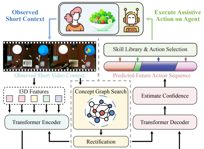
Fig. 1: NeSCA: Given a short video segment (blue), our system anticipates future actions and their respective confidences (color gradients) utilizing our proposed neuro-symbolic attention approach to re-focus attention between visual features. Finally, if sufficiently confident about the prediction, a robot executes assistive actions (green).
